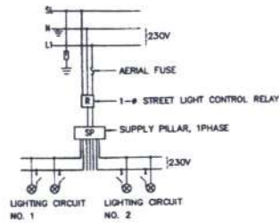
BLOCK DIAGRAM 1
