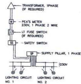
BLOCK DIAGRAM 3
