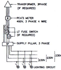
BLOCK DIAGRAM 2
