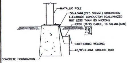
GROUNDING DETAILS NOT TO SCALE
