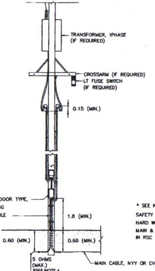
BLOCK DIAGRAM 3
