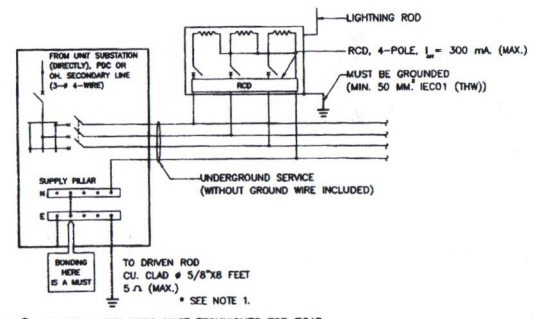
METHOD C: LIGHTING WITH HIGH-MAST TECHNIQUES FOR ROAD (LIGHTING POLE/COLUMN ACCESSIBLE TO PUBLIC)
