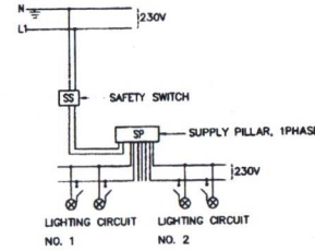
BLOCK DIAGRAM 2
