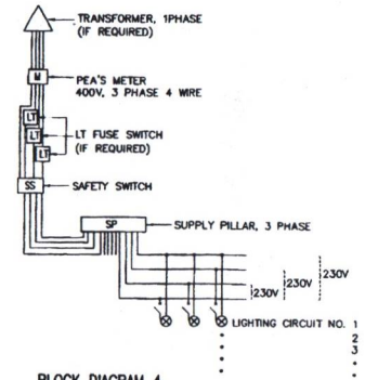
BLOCK DIAGRAM 4
