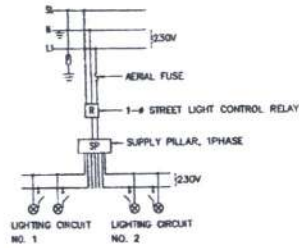
BLOCK DIAGRAM 1
