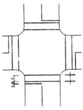
STANDARD CROSSWALK MARKING CROSSWALK MARKINGS NOT TO SCALE
