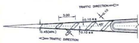
CROSS HATCHING MARKING NOT TO SCALE
