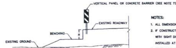
BENCHING ROAD CONSTRUCTION NOT TO SCALE
