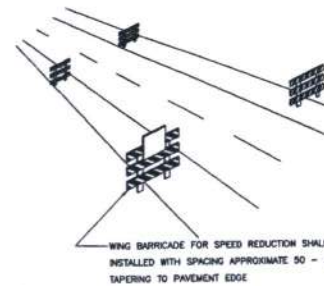
WING BARRICADE FOR SPEED REDUCTION SHALL BE INSTALLED WITH SPACING APPROXIMATE 50 - 100 M. TAPERING TO PAVEMENT EDGE SPEED CONTROL SIGN NOT TO SCALE
