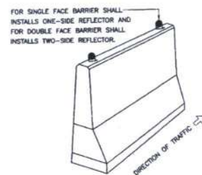
INSTALLATION REFLECTIVE TARGET ON BARRIER NOT TO SCALE
