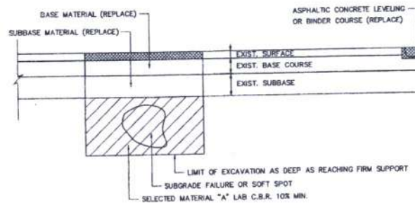
SECTION OF LOCALIZED FAILURE
