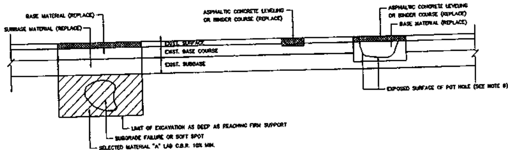
SECTION OF POT HOLE
