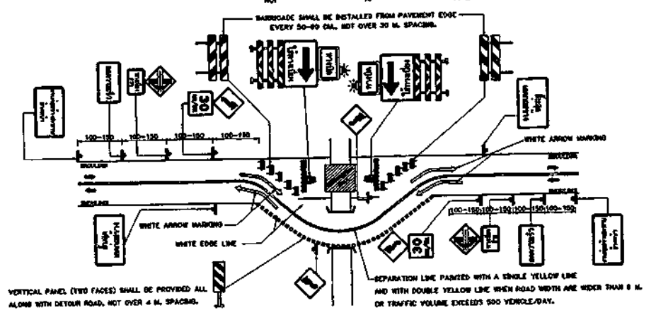
DETOUR BRIDGE OR TWO-LANE DETOUR ROAD NOT TO SCALE
