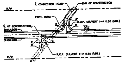
CONNECTION ROAD, \theta BETWEEN 45°-60° NOT TO SCALE
