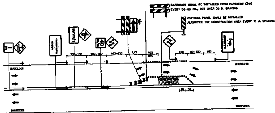
A. FOUR-LANE HIGHWAYS NOT TO SCALE
