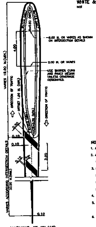
MARKING AT ISLAND NOT TO SCALE
