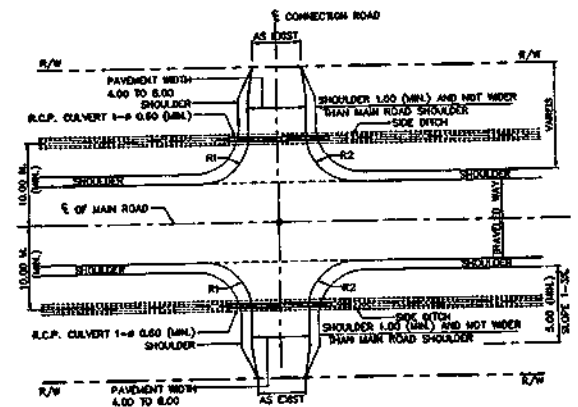
CONNECTION ROAD PLAN NOT TO SCALE
