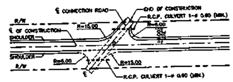
CONNECTION ROAD, \theta BETWEEN 45°-60° NOT TO SCALE
