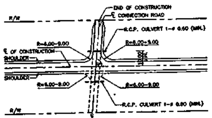
CONNECTION ROAD, \theta BETWEEN 80°-90° NOT TO SCALE
