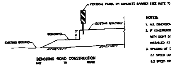
FOUR - LANE HIGHWAYS CONSTRUCTION WITHOUT MEDIAN, MIDWAY CLOSED NOT TO SCALE
