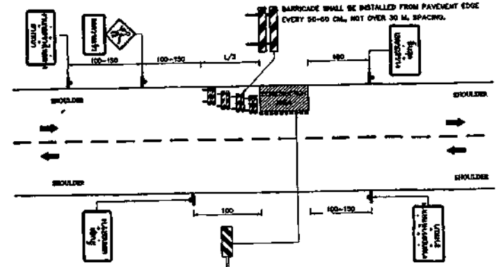
WORK ON THE SHOULDER NOT TO SCALE
