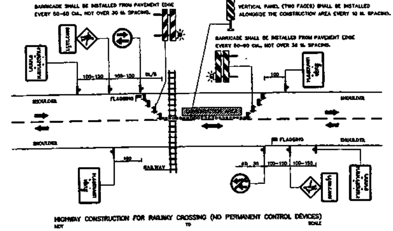
FOR ONE WAY TRAFFIC CONSTRUCTION NOT TO SCALE
