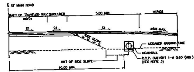
CONNECTION ROAD SECTION NOT TO SCALE
