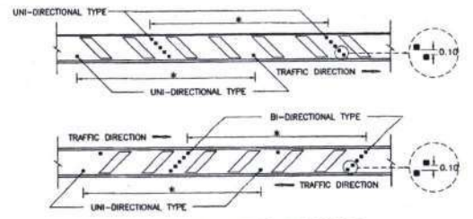
ROAD STUD AT CROSS HATCHING NOT TO SCALE
