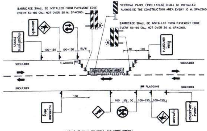
FOR ONE WAY TRAFFIC CONSTRUCTION NOT TO SCALE
