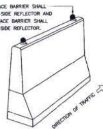
INSTALLATION REFLECTIVE TARGET ON BARRIER NOT TO SCALE
