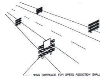
WING BARRICADE FOR SPEED REDUCTION SHALL BE INSTALLED WITH SPACING APPROXIMATE 50 - 100 M. TAPERING TO PAVEMENT EDGE
