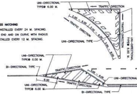
ROAD STUD AT ISLAND MARKINGS NOT TO SCALE
