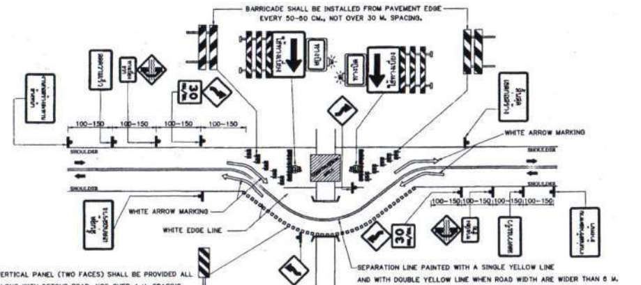
DETOUR BRIDGE OR TWO-LANE DETOUR ROAD NOT TO SCALE
