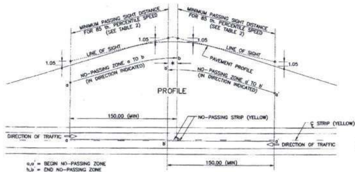
CENTER LINE MARKING FOR NO-PASSING ZONES AT VERTICAL CURVES NOT TO SCALE
