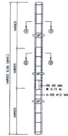
REINFORCE CONCRETE POST DETAIL NOT TO SCALE
