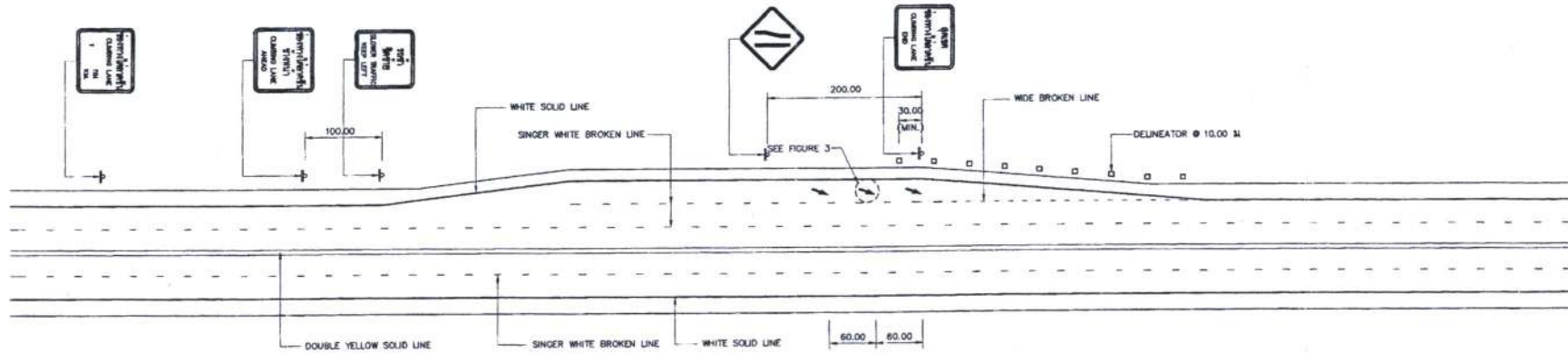
FIGURE 2 INSTALLATION TRAFFIC SIGN ON CLIMBING LANE FOR MULTI-LANE HIGHWAYS (ONLY LEFT SIDE OF TRAFFIC DIRECTION)
