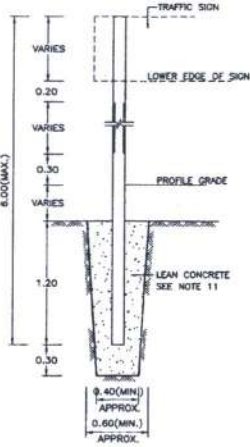
SIGN POST INSTALLATION DETAIL NOT TO SCALE
