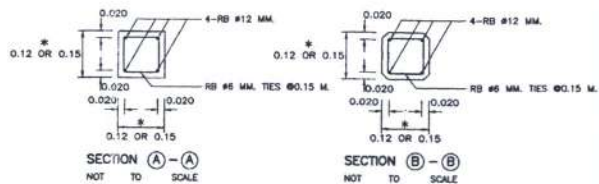
SECTION A-A NOT TO SCALE SECTION B-B NOT TO SCALE
