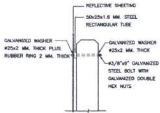
TYPICAL FIXING OF SIGN PLATE
