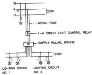
BLOCK DIAGRAM 1
