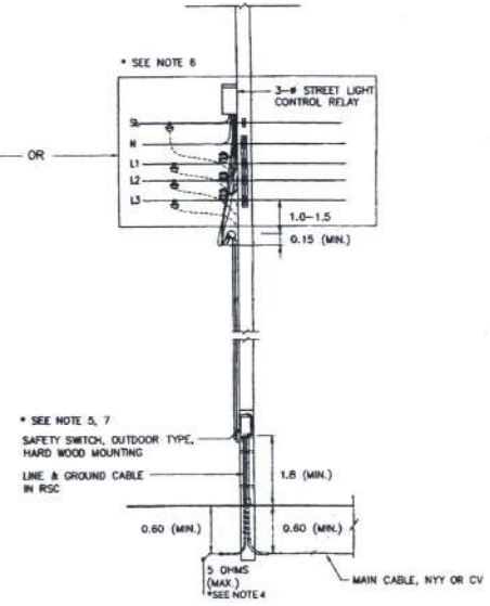
TYPE 3: FOR MEA'S OVERHEAD LINE, 3PH 4WIRE, IN OR NOT IN THE AREA OF UNDERGROUND CABLE PROJECT
