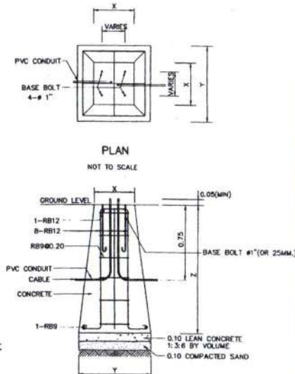
LIGHTING POLE FOUNDATION DETAILS NOT TO SCALE
