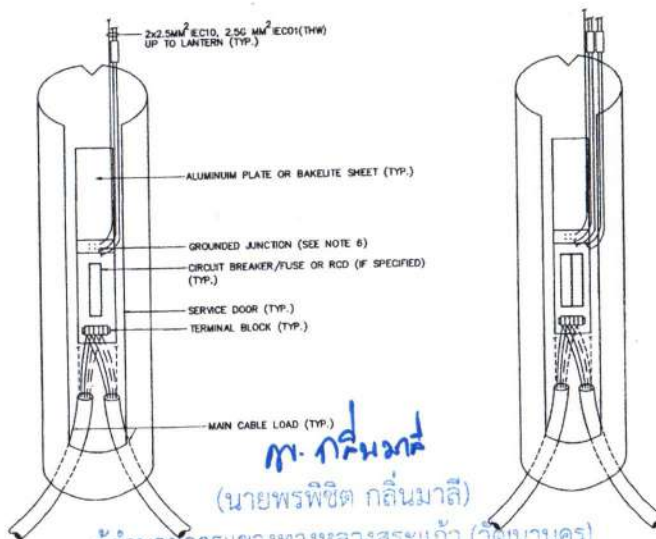
TYPE 2: FOR LIGHTING POLE, DOUBLE ARM(2 PHASE)
