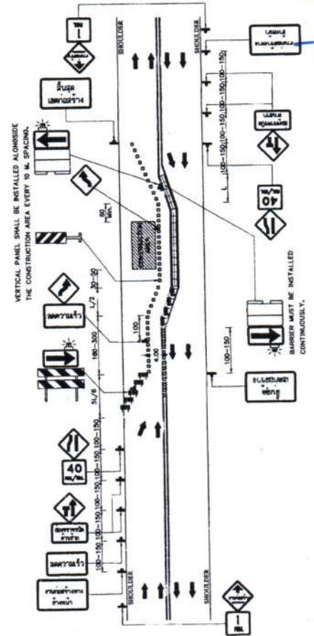
FOUR - LANE HIGHWAYS CONSTRUCTION WITHOUT MEDIAN, ONE WAY CLOSED SCALE
