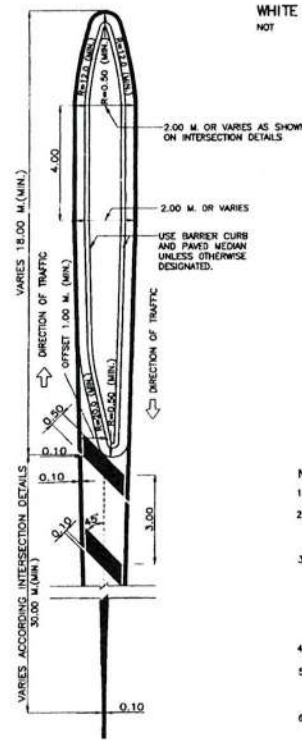
MARKING AT ISLAND NOT TO SCALE
