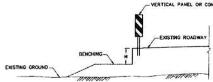
BENCHING ROAD CONSTRUCTION NOT TO SCALE
