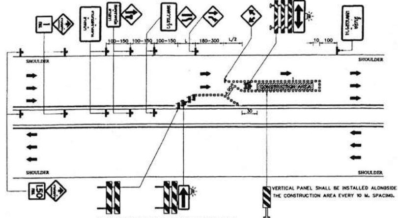
BARRICADE SHALL BE INSTALLED FROM PAVEMENT EDGE EVERY 50-60 CM., NOT OVER 30 M. SPACING.
