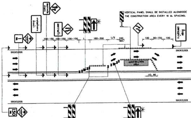
B. SIX-LANE HIGHWAYS WITH SHOULDER, MIDDLE LANE CLOSED NOT TO SCALE
