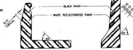
MARKING AT ENDS OF BRIDGE BARRIER NOT TO SCALE
