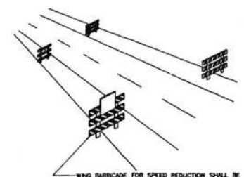
WING BARRICADE FOR SPEED REDUCTION SHALL BE INSTALLED WITH SPACING APPROXIMATE 50 - 100 M. TAPERING TO PAVEMENT EDGE
