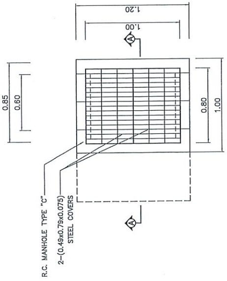
PLAN OF R.C. MANHOLE TYPE "C"
