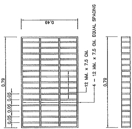
PLAN OF R.C. MANHOLE TYPE "C"
