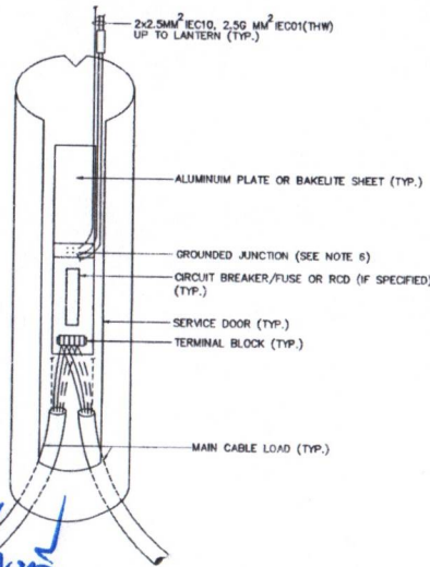
TYPE1: FOR LIGHTING POLE, SINGLE ARM OR DOUBLE ARM(1 PHASE)
