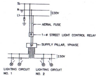
BLOCK DIAGRAM 1
