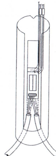
TYPE 2: FOR LIGHTING POLE, DOUBLE ARM(2 PHASE)
