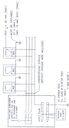
METHOD ② : LIGHTING WITHOUT HIGH-MAST TECHNIQUES FOR GROUND-LEVEL ROAD (LIGHTING POLE/COLUMN ACCESSIBLE TO PUBLIC)
