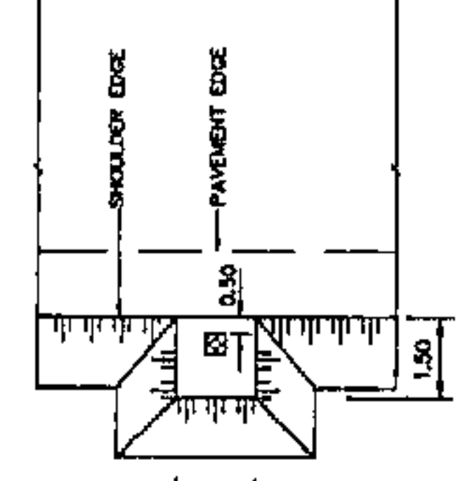
LOCATION OF LIGHTING POLE, AT GRADE NOT TO SCALE
