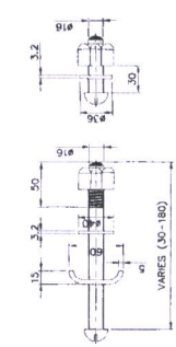
BOLT & NUT SCALE 1:1.3
