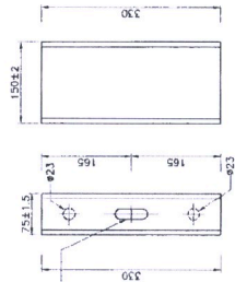
FRONT VIEW SIDE VIEW
