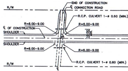
CONNECTION ROAD, \theta BETWEEN 80°-90° NOT TO SCALE
