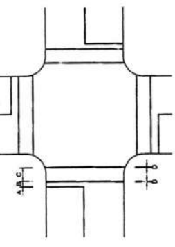
STANDARD CROSSWALK MARKING NOT TO SCALE
