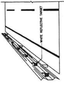
INSTALLATION REFLECTIVE TARGET ON GUARDRAIL SCALE TO NOT
