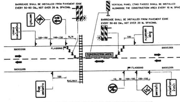
HIGHWAY CONSTRUCTION FOR RAILWAY CROSSING (NO PERMANENT CONTROL DEVICES) NOT TO SCALE
