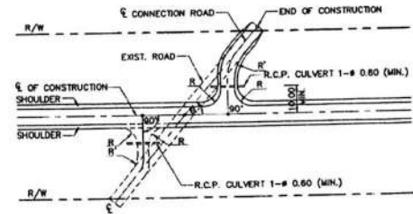
CONNECTION ROAD, \theta BETWEEN 45°-60° NOT TO SCALE
