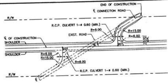
CONNECTION ROAD, \theta LESS THAN 45° NOT TO SCALE
