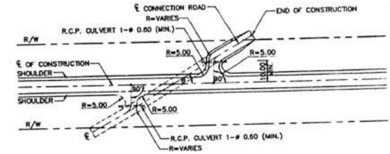
CONNECTION ROAD, \theta LESS THAN 45° NOT TO SCALE
