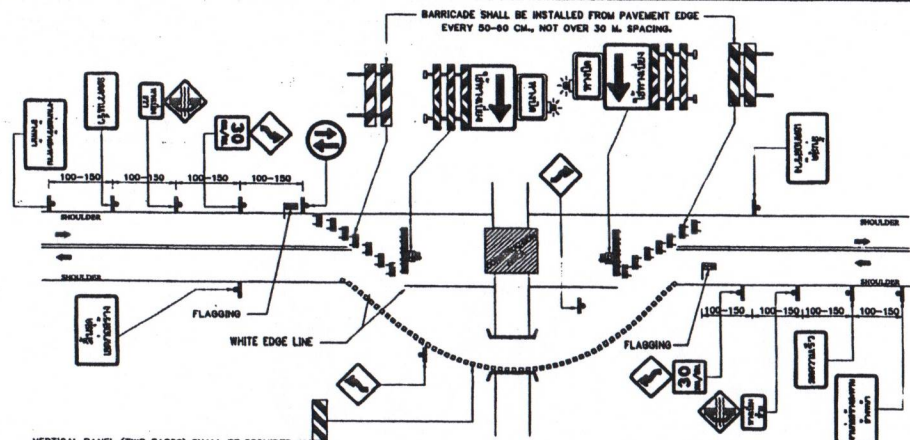
DETOUR BRIDGE OR ONE-LANE DETOUR ROAD NOT TO SCALE
