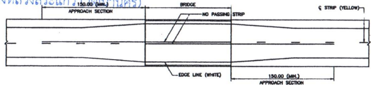
MARKING AT BRIDGE APPROACH NOT TO SCALE
