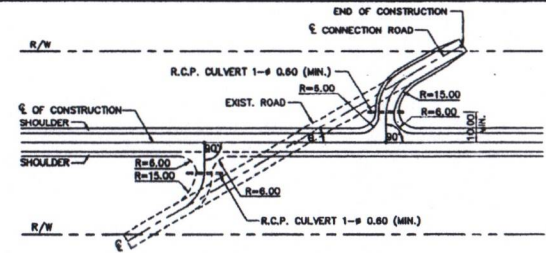
RIGHT OF WAY WIDTH > 20.00 M. CONNECTION ROAD, \theta LESS THAN 45° NOT TO SCALE
