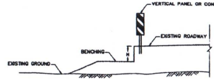
BENCHING ROAD CONSTRUCTION NOT TO SCALE
