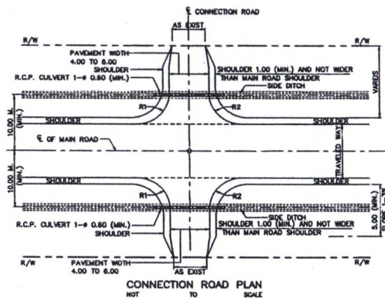
CONNECTION ROAD, \theta BETWEEN 60°-80° NOT TO SCALE
