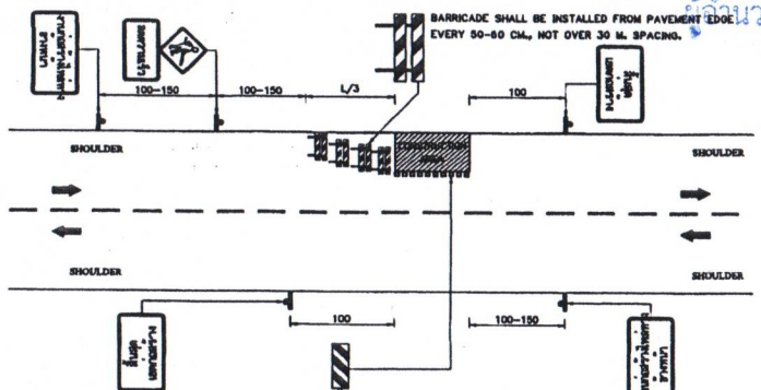
WORK ON THE SHOULDER NOT TO SCALE
