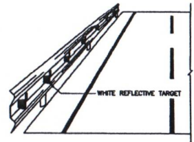
INSTALLATION REFLECTIVE TARGET ON GUARDRAIL NOT TO SCALE
