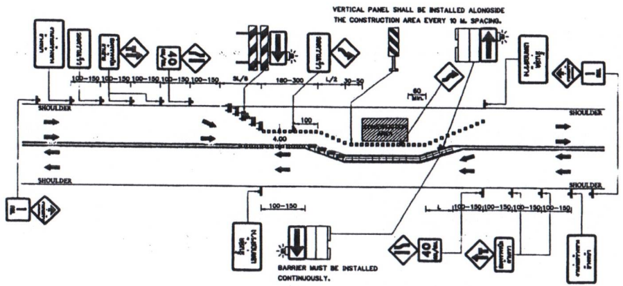
FOUR - LANE HIGHWAYS CONSTRUCTION WITHOUT MEDIAN, ONE WAY CLOSED NOT TO SCALE
