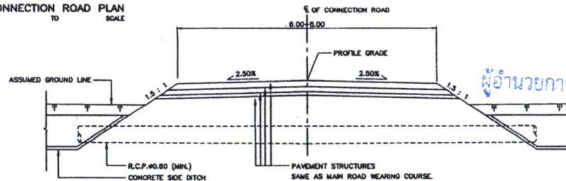
TYPICAL CROSS-SECTION FOR CONNECTION ROAD SCALE 1 : 100
