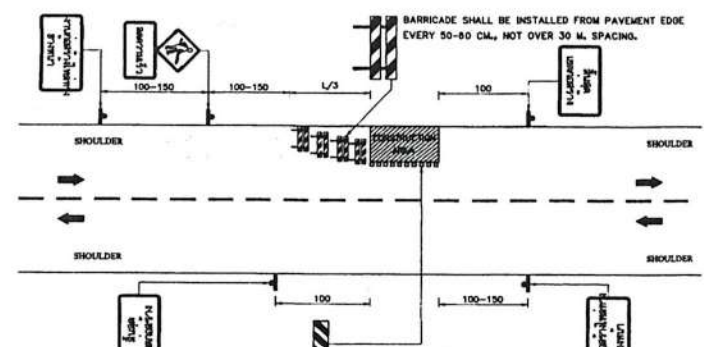
WORK ON THE SHOULDER NOT TO SCALE
