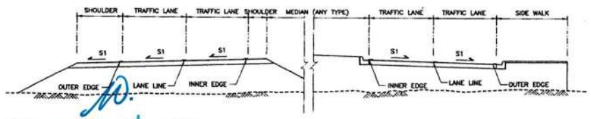
MARKING AT PAVEMENT NOT TO SCALE
