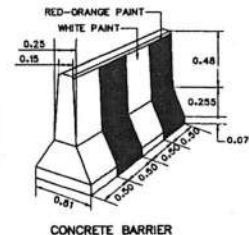
CONCRETE BARRIER
