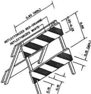
BARRICADE TYPE I NOT TO SCALE
