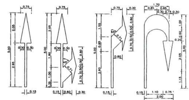
DIRECTIONAL ARROWS NOT TO SCALE
