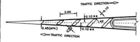
CROSS HATCHING MARKING NOT TO SCALE
