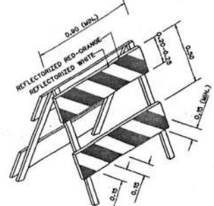
BARRICADE TYPE I NOT TO SCALE
