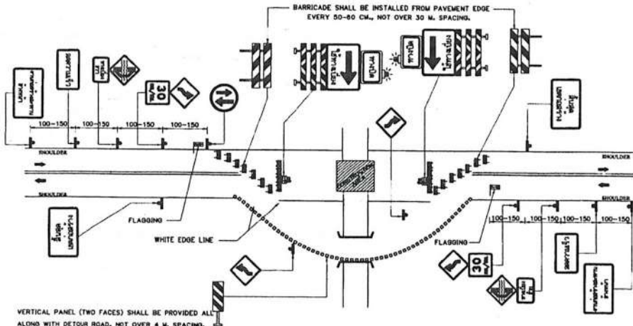
DETOUR BRIDGE OR ONE-LANE DETOUR ROAD NOT TO SCALE
