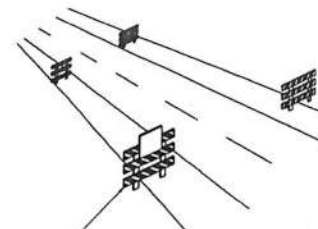
WING BARRICADE FOR SPEED REDUCTION SHALL BE INSTALLED WITH SPACING APPROXIMATE 50 - 100 M. TAPERING TO PAVEMENT EDGE
