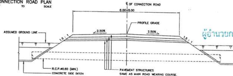
TYPICAL CROSS-SECTION FOR CONNECTION ROAD SCALE 1 : 100
