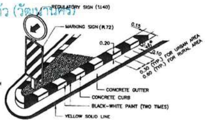
MARKING AT ENDS OF BRIDGE BARRIER NOT TO SCALE
