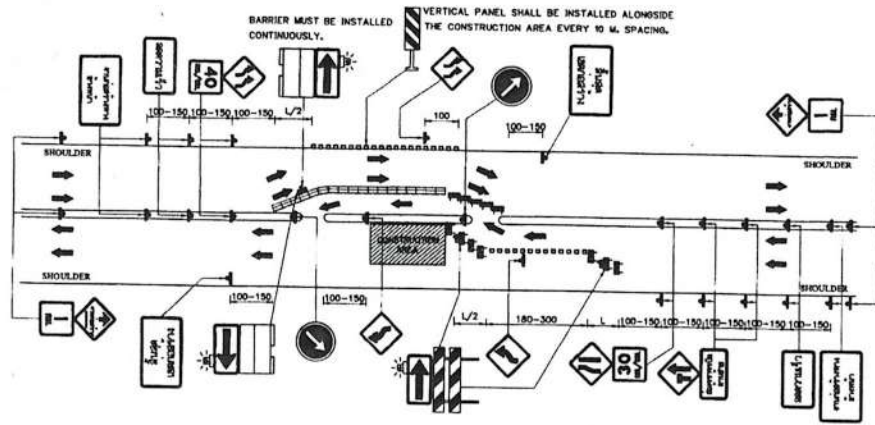
DIVIDED HIGHWAYS CONSTRUCTION, ONE WAY CLOSED NOT TO SCALE
