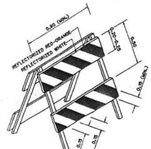
BARRICADE TYPE I NOT TO SCALE
