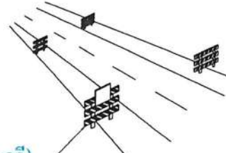
WIND BARRICADE FOR SPEED REDUCTION SHALL BE INSTALLED WITH SPACING APPROXIMATE 50 - 100 M. STARTING TO PAVEMENT EDGE SPEED CONTROL SIGN NOT TO SCALE
