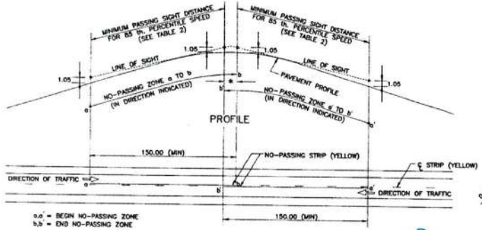
PROFILE PLAN
