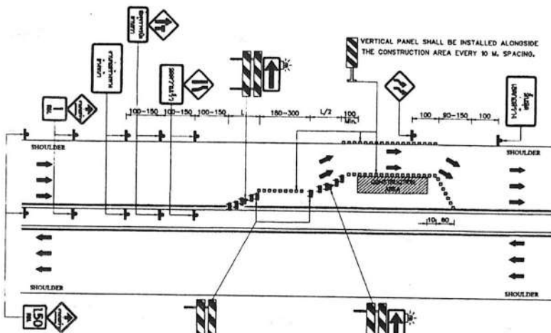
A. FOUR-LANE HIGHWAYS NOT TO SCALE
