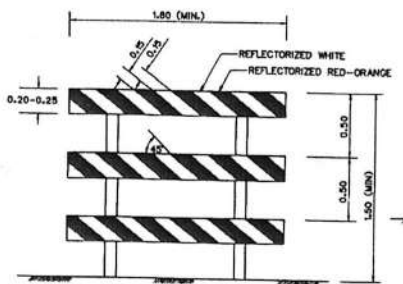
BARRICADE TYPE II NOT TO SCALE
