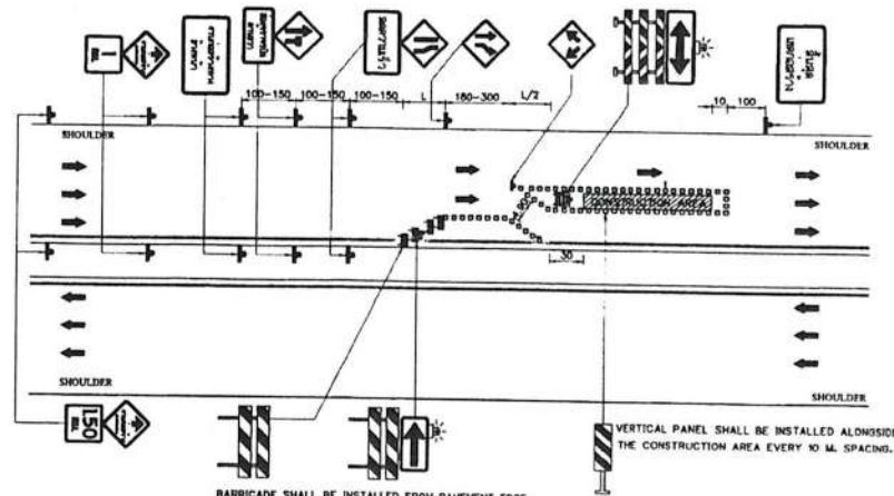
B. SIX-LANE HIGHWAYS WITH SHOULDER, MIDDLE LANE CLOSED NOT TO SCALE
