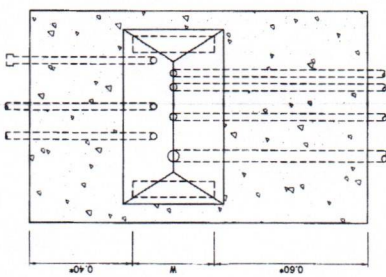
SUPPLY PILLAR ON CONCRETE POLE NOT TO SCALE
