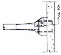
SECTION D-D NOT TO SCALE
