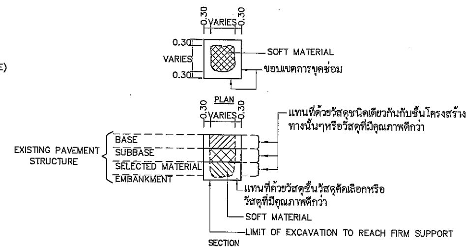
SOFT MATERIAL EXCAVATION AND REPLACEMENT
