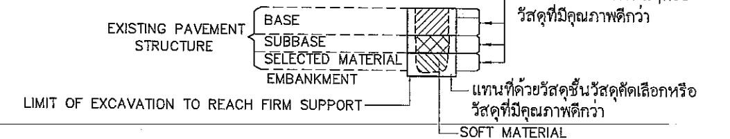
SECTION
