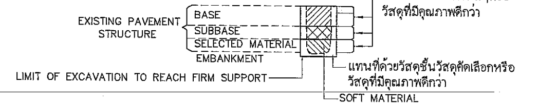
SECTION
