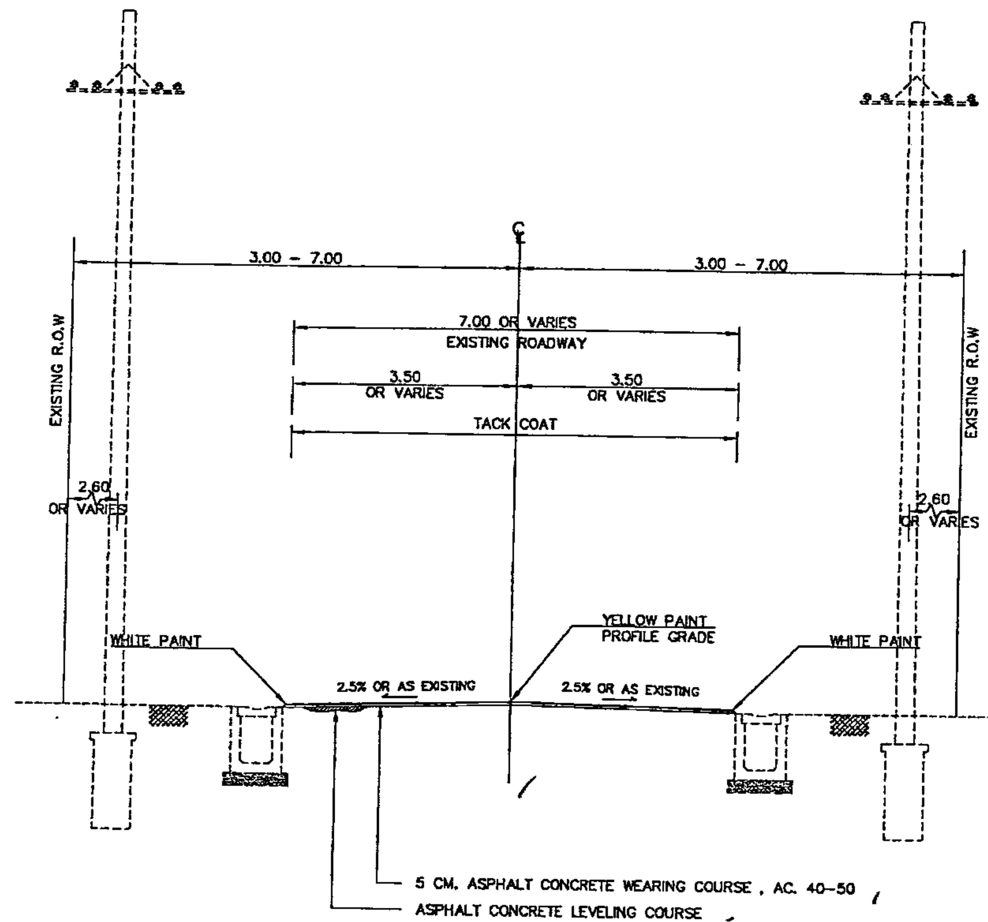
TYPICAL CROSS SECTION II SCALE 1:100 กม.31+490 - กม.32+900
