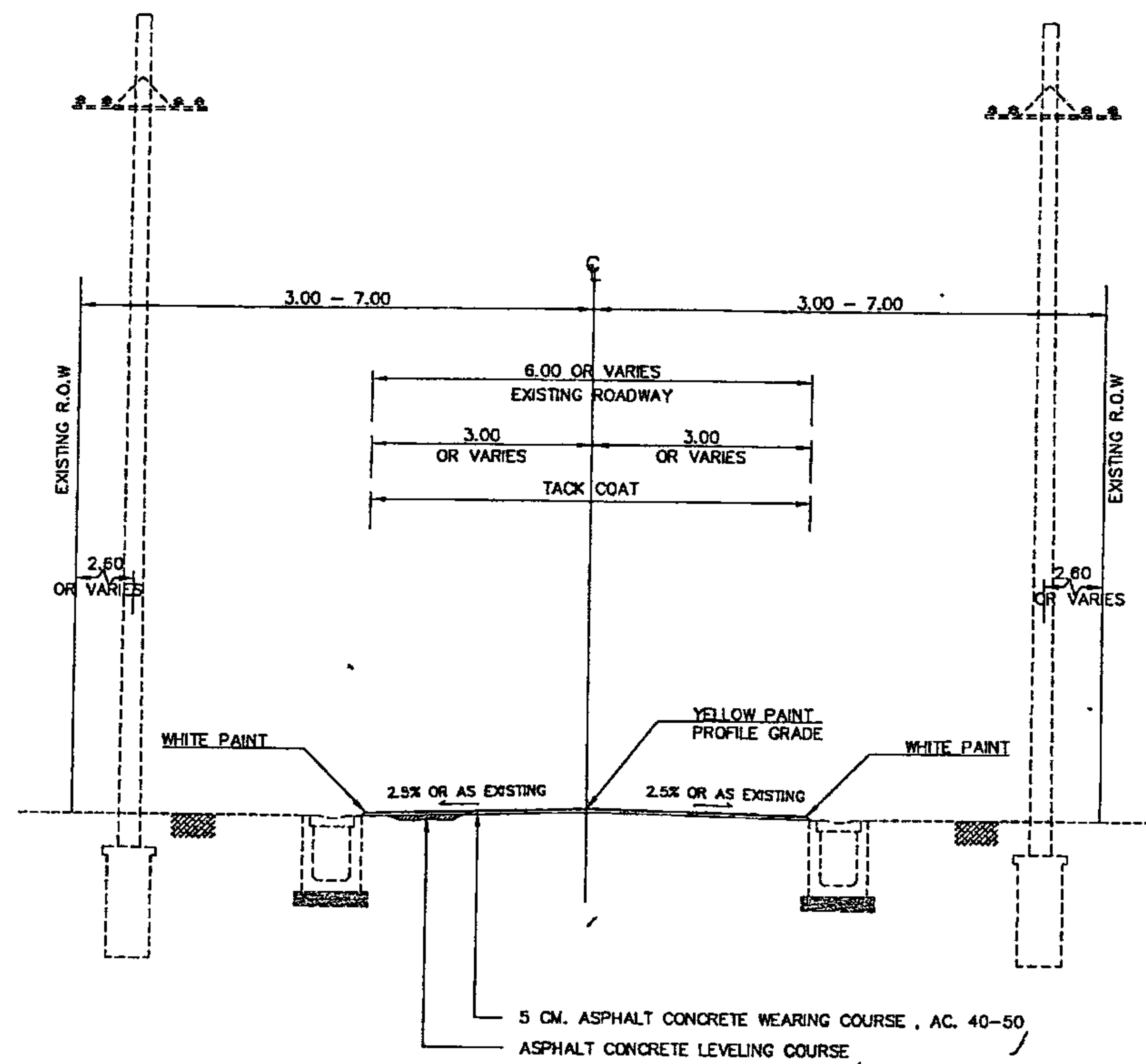
TYPICAL CROSS SECTION III SCALE 1:100 กม.32+900 - กม.33+825
