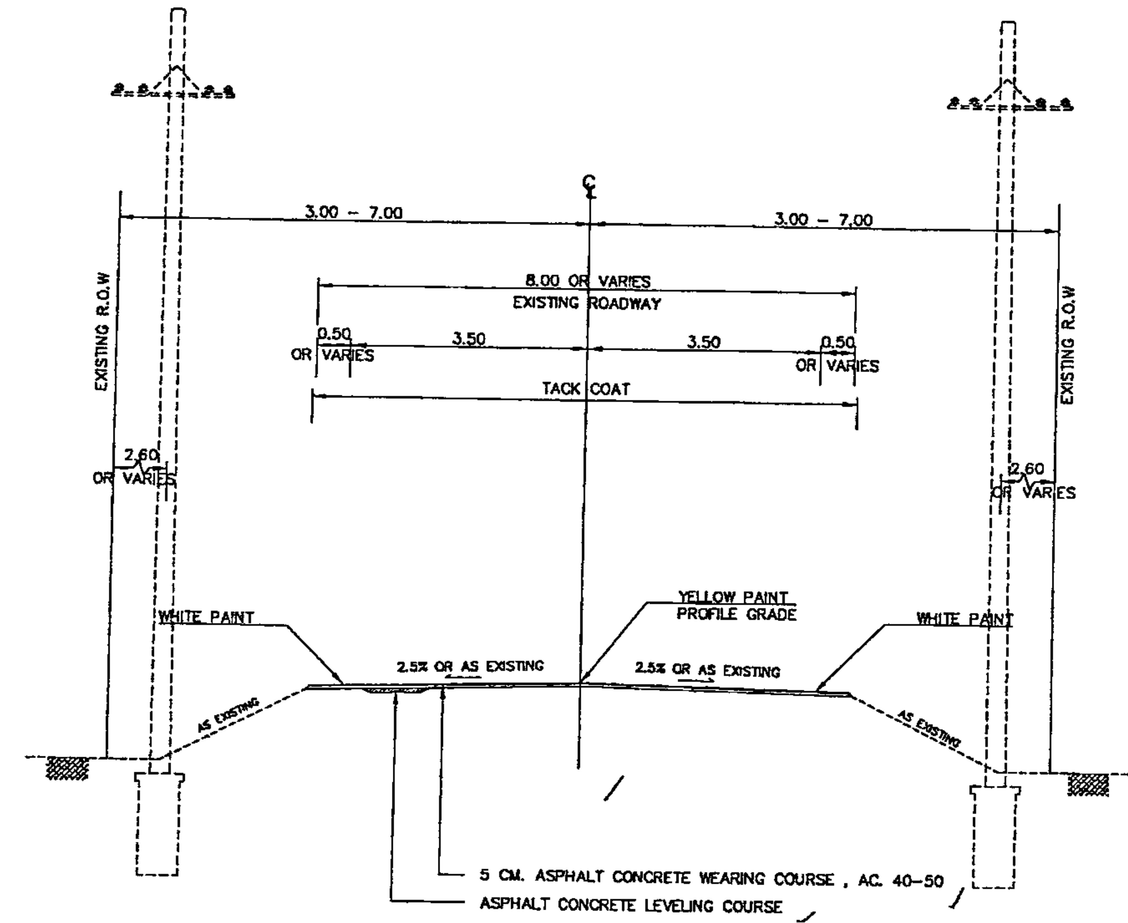
TYPICAL CROSS SECTION 1 SCALE 1:100 กม.31+140 - กม.31+490
