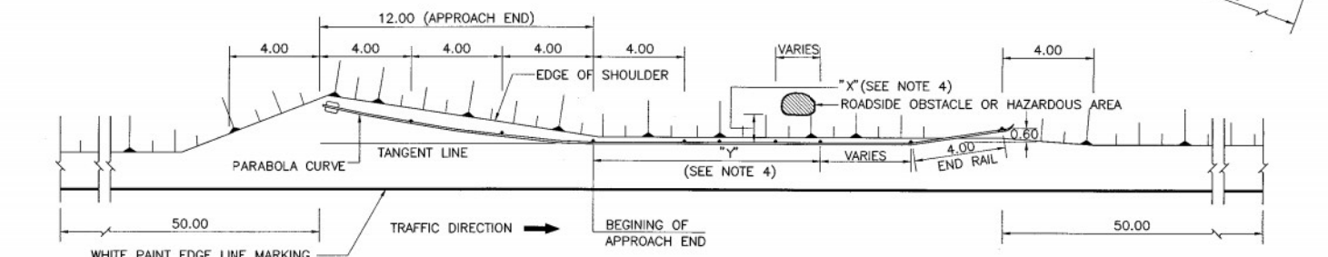
APPROACH END INSTALLATION FOR ROADSIDE OBSTACLE
