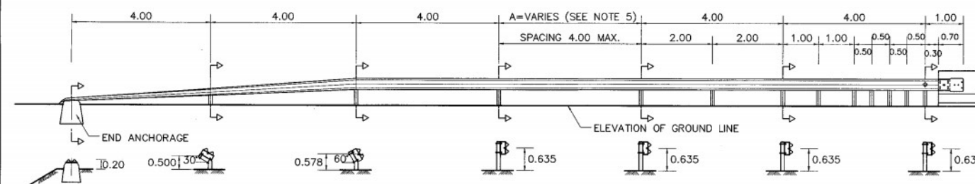
ELEVATION OF GUARDRAIL CONNECTION TO BRIDGE RAILING
