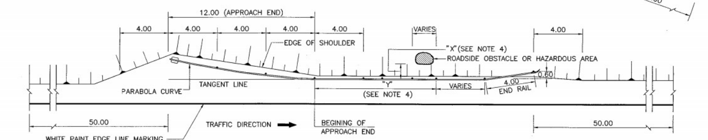
APPROACH END INSTALLATION FOR ROADSIDE OBSTACLE
