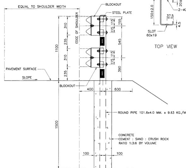
PLAN AND SECTION NOT TO SCALE
