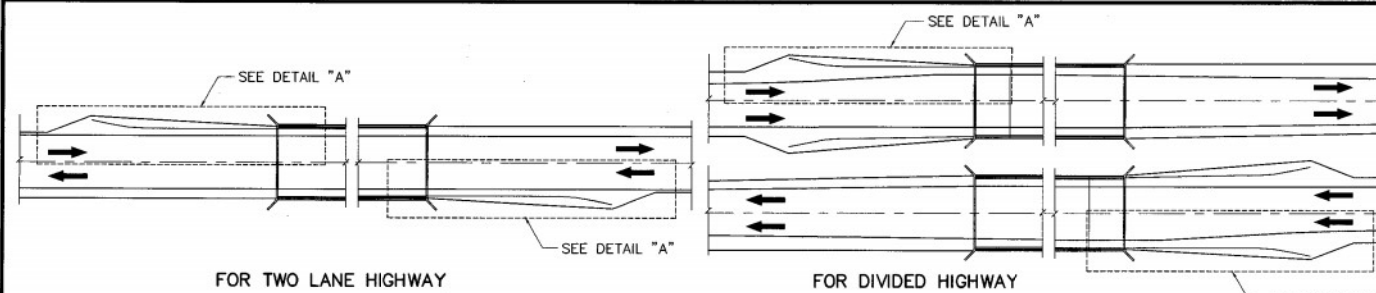
INSTALLATION OF W-BEAM GUARDRAIL AT BRIDGE APPROACH PLAN SCALE 1 : 500
