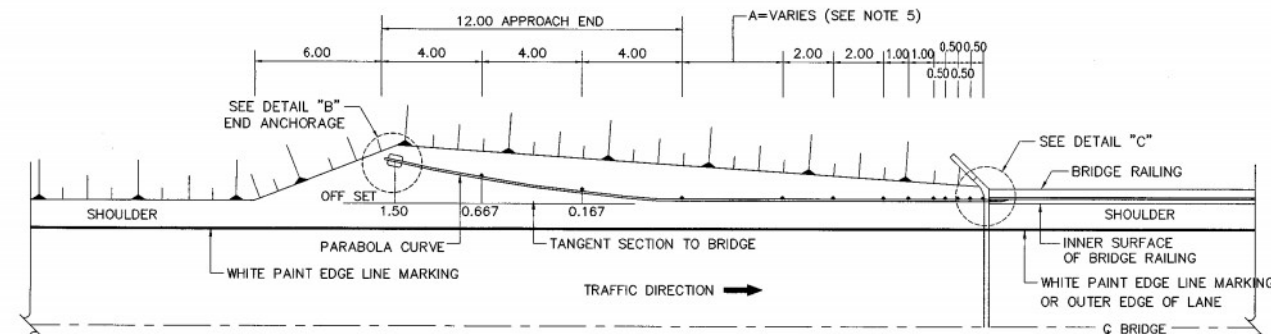
DETAIL "A" WITHOUT BRIDGE SIDEWALK
