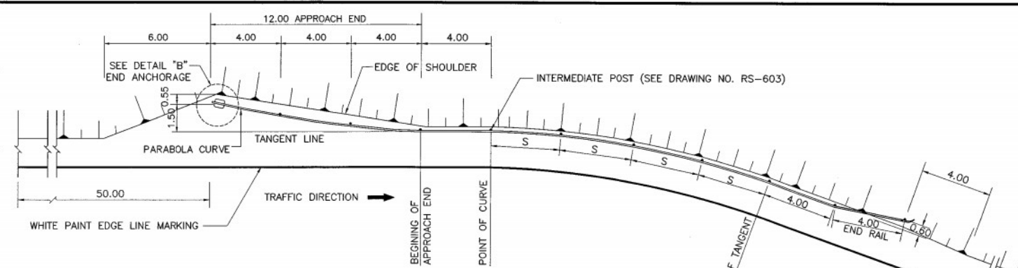
INSTALLATION OF W-BEAM GUARDRAIL AT HORIZONTAL CURVE
