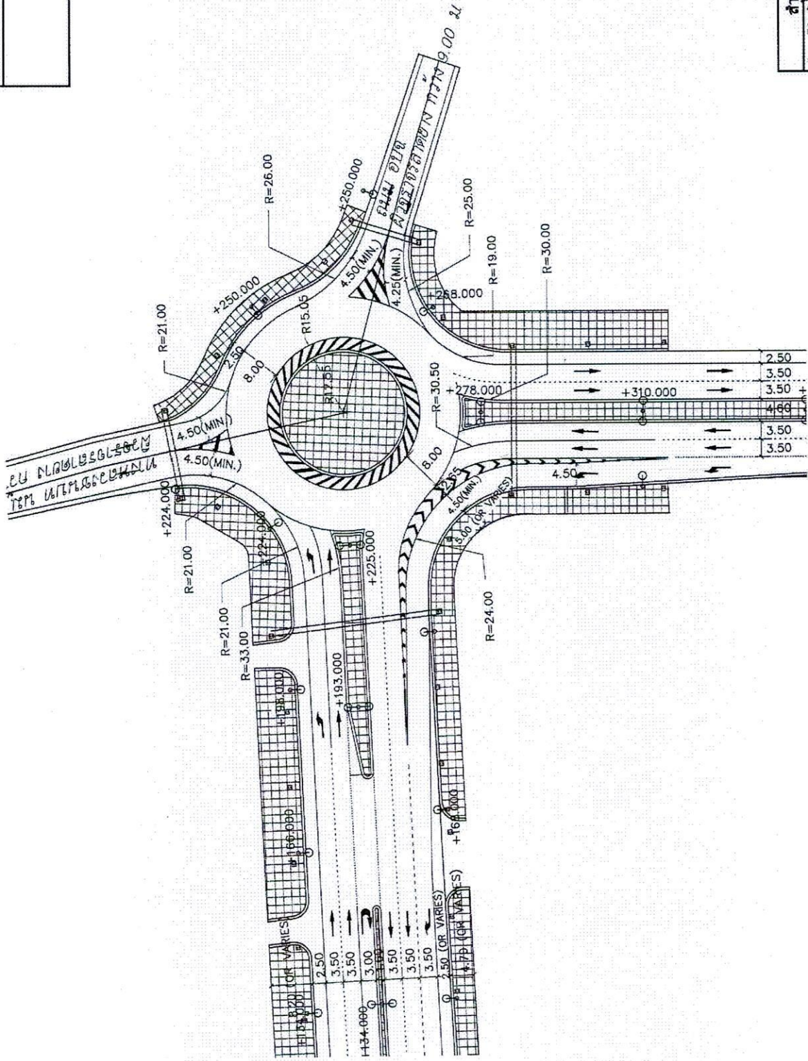
DETAIL OF ROUNDABOUT NOT TO SCALE
