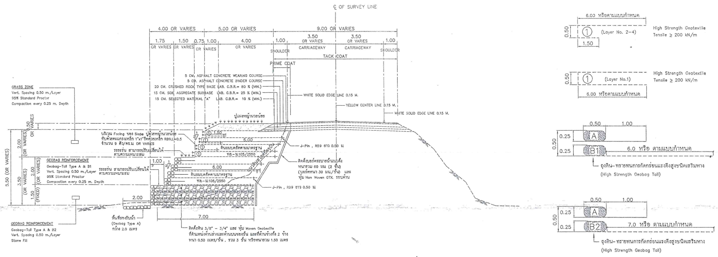
TYPICAL CROSS SECTION (5) SCALE 1 : 150
