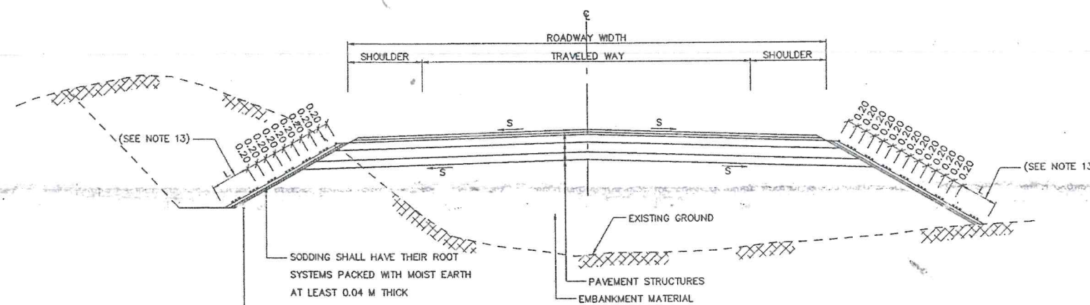
STRIP SODDING NOT TO SCALE
