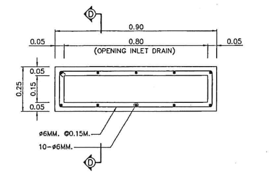
SECTION (C) - (C) RECTANGULAR DRAINAGE PIPE SCALE 1 : 10
