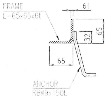
DETAIL ADD ANCHOR Round bar Ø9x150L (SECTION "C")
