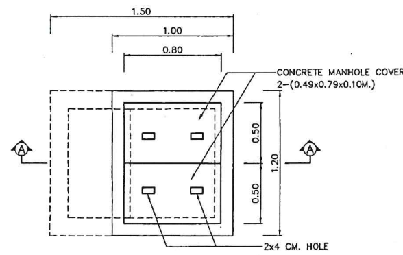
PLAN OF MANHOLE TYPE "C" SCALE 1 : 20
