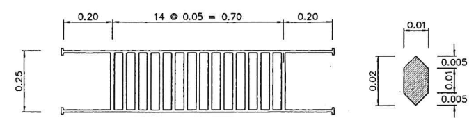
CAST-IRON GRATING DETAILS SCALE 1 : 10
