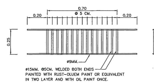
STEEL GRATING DETAILS SCALE 1 : 10
