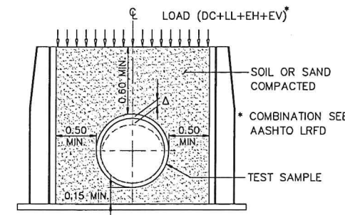
GUIDELINES FULL SCALE MODEL TEST SCALE NON
