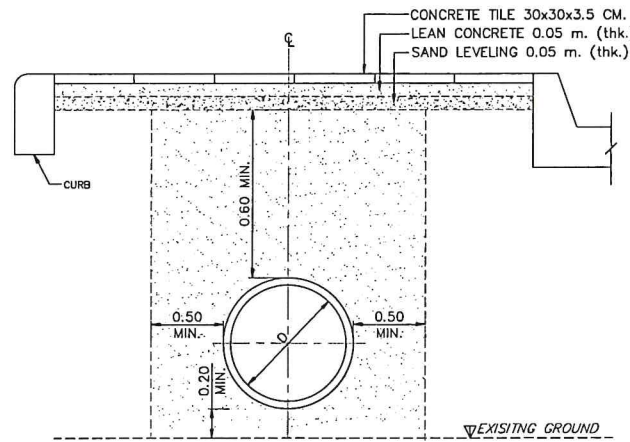
CASE III : ROCK OR UNYIELDING FOUNDATION INSTALLATION BY TRENCH METHOD SCALE NON
