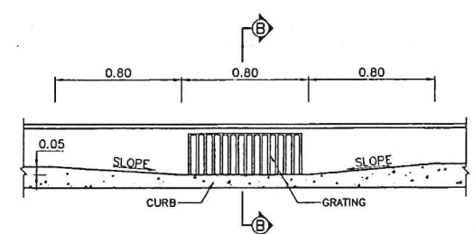
FRONT VIEW FOR INLET DRAIN SCALE 1 : 20
