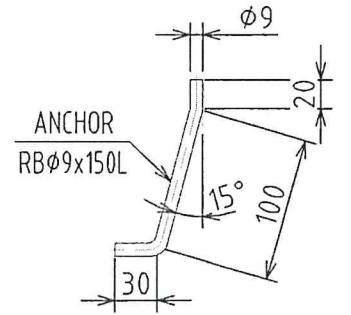
DETAIL OF ANCHOR RBØ9x150L
