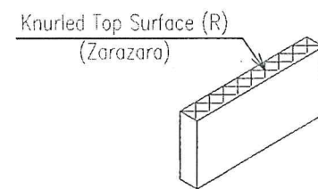
DETAIL OF KNURLED FLAT BAR (R = KNURLING)
