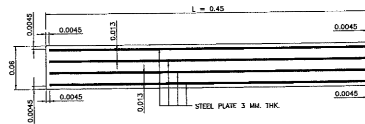
SECTION B - B BEARING TYPE "FR" SCALE 1 : 25
