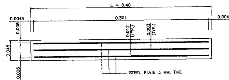
SECTION A - A BEARING TYPE "FR" SCALE 1 : 25
