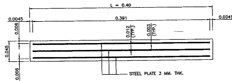
SECTION A - A BEARING TYPE "FX" SCALE 1 : 25
