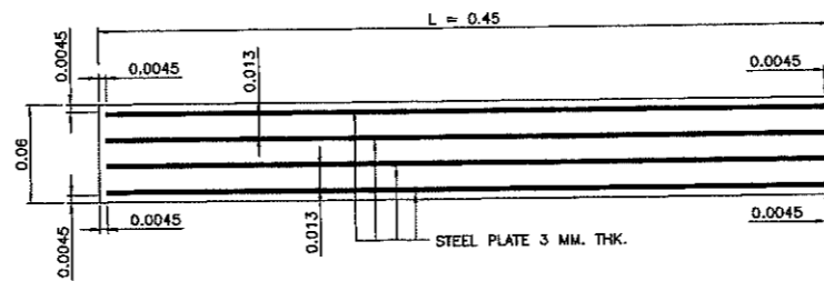
SECTION B - B BEARING TYPE "FX" SCALE 1 : 25
