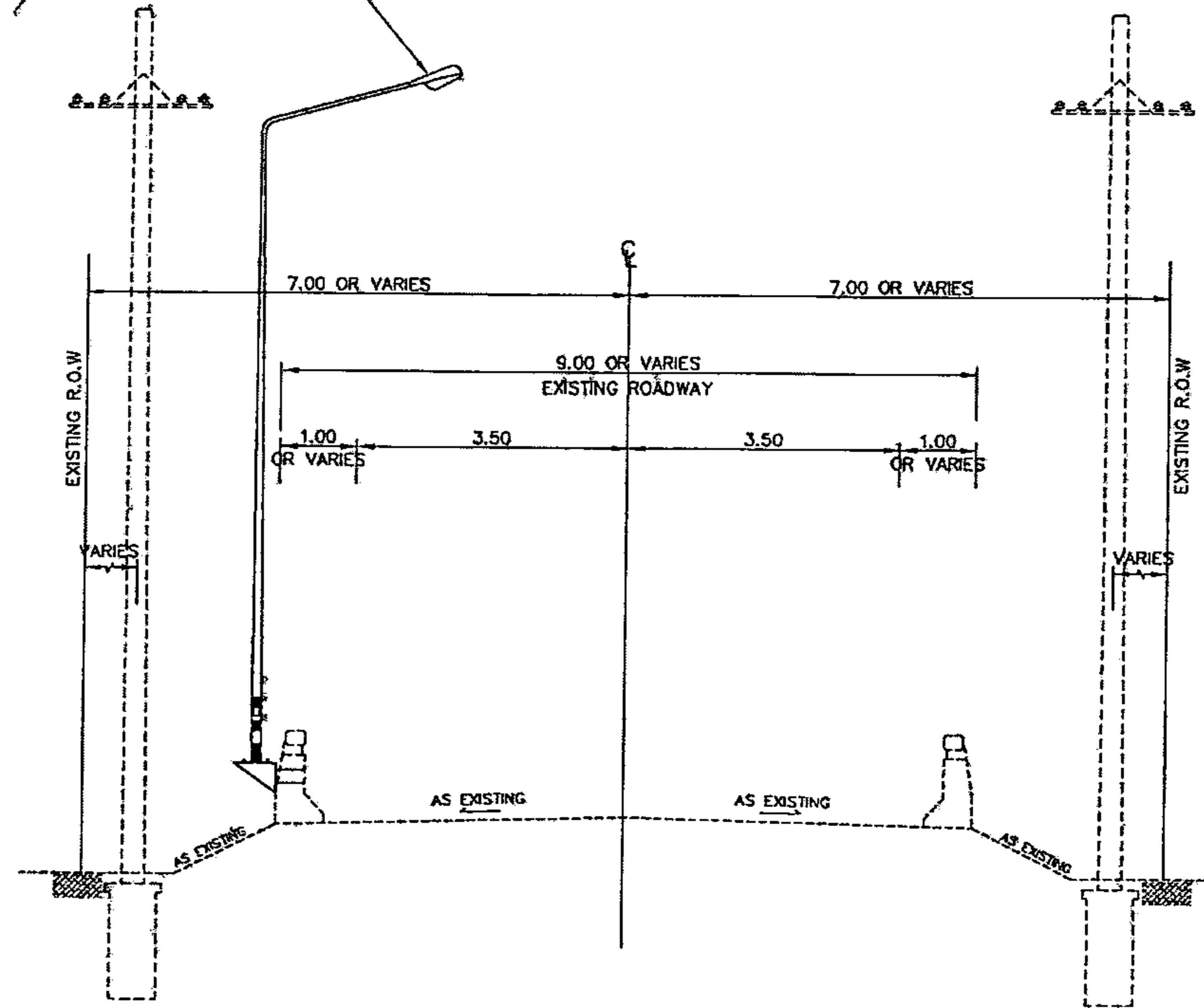
TYPICAL CROSS SECTION II
