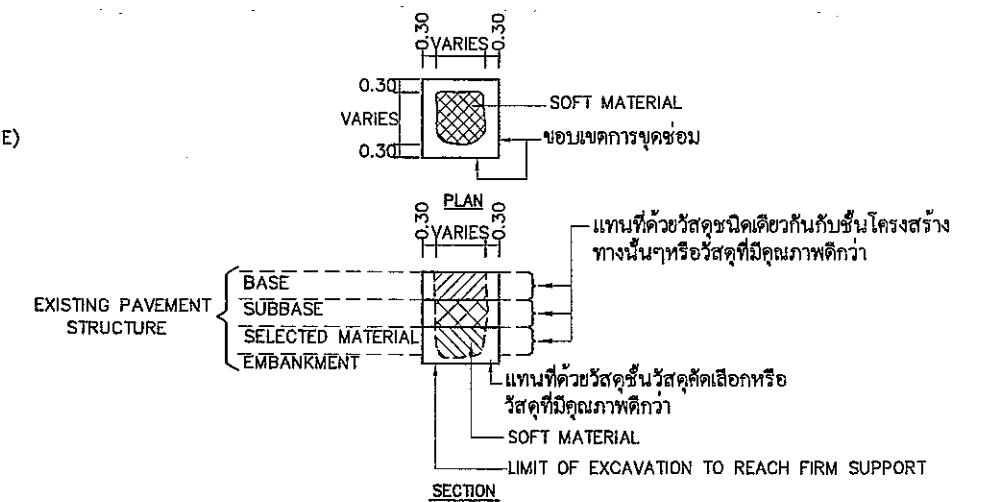
SOFT MATERIAL EXCAVATION AND REPLACEMENT
