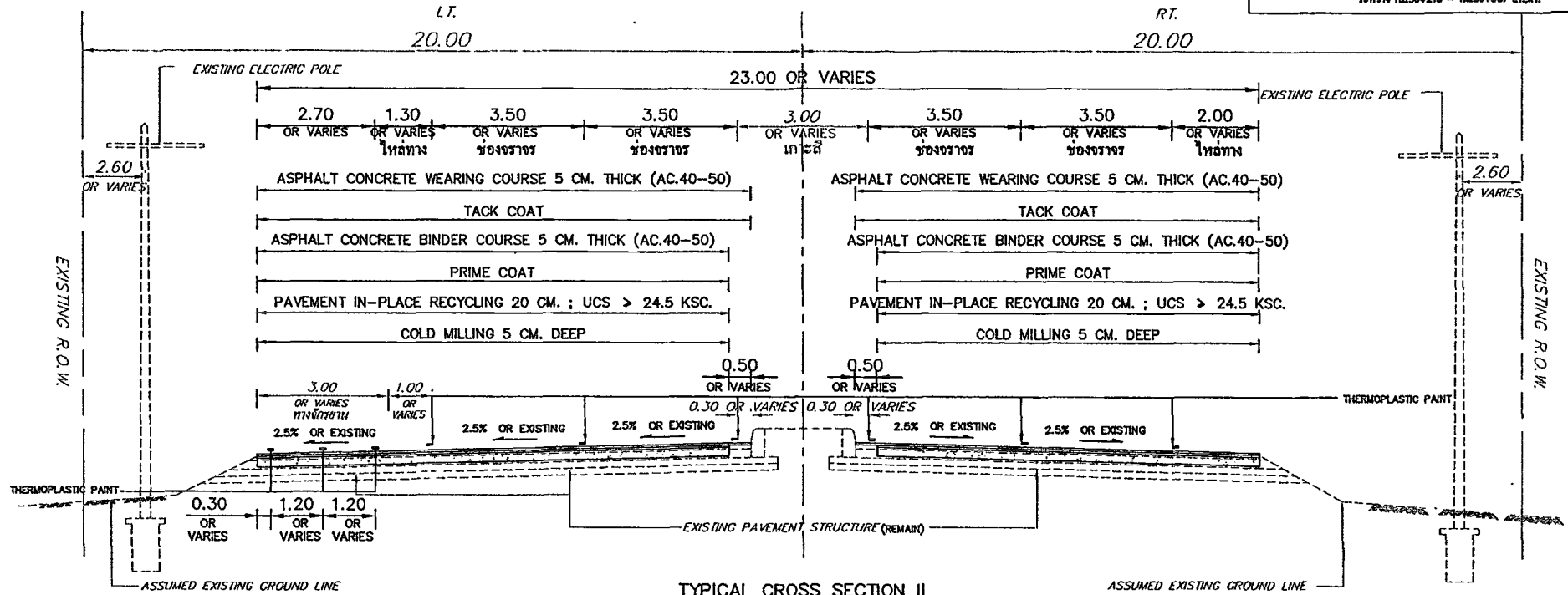
TYPICAL CROSS SECTION II
