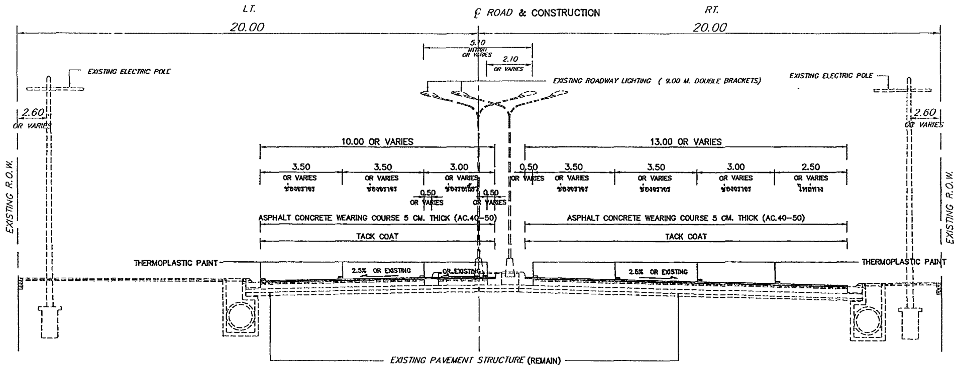
TYPICAL CROSS SECTION III
