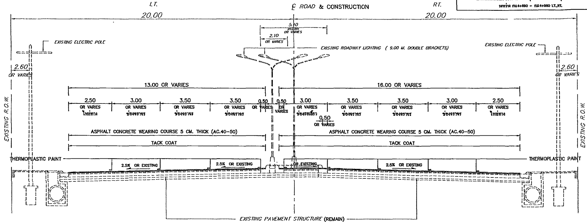
TYPICAL CROSS SECTION I
