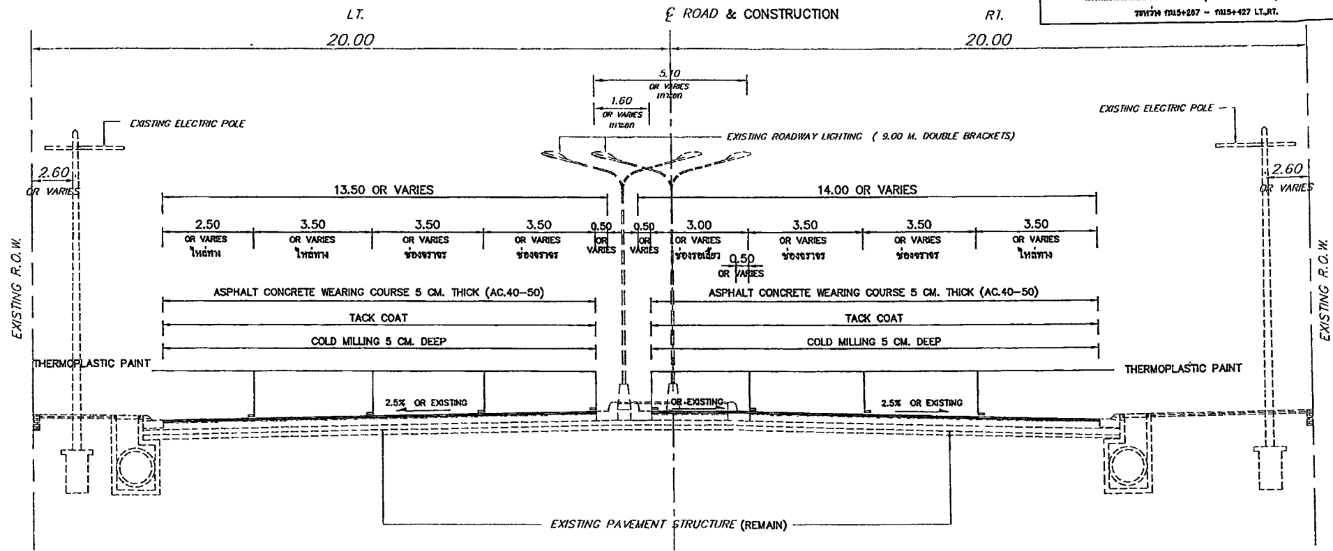
TYPICAL CROSS SECTION IV
