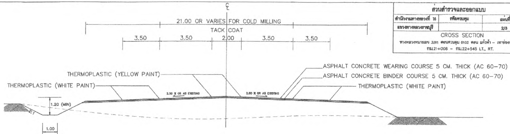
TYPICAL CROSS SECTION SCALE 1:100
