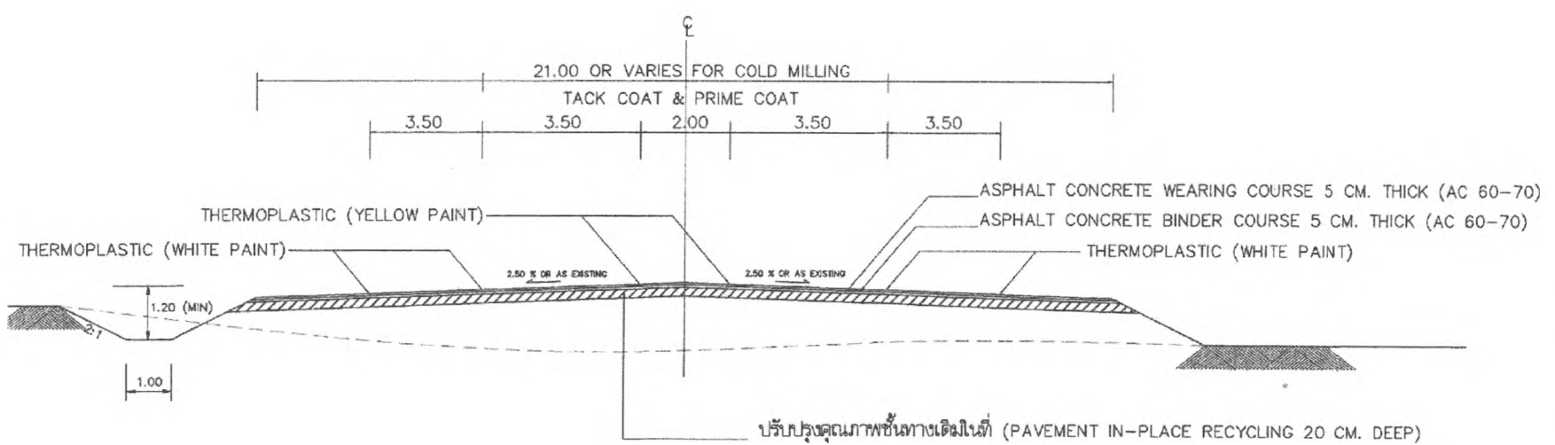
TYPICAL CROSS SECTION SCALE 1:100
