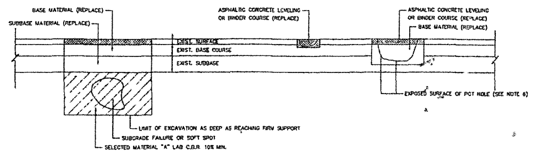
SECTION OF LOCALIZED FAILURE
